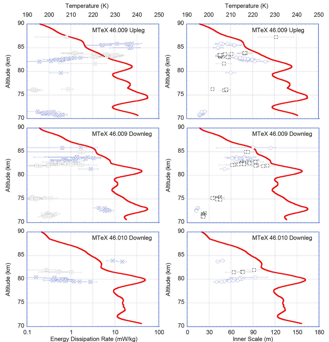
Figure 10. Temperature (solid red), turbulent energy dissipation rate (blue square with x and black square with +), and turbulent inner scale (blue circle and black circle in square) derived from MTEx CONE ion gauge measurements plotted as function of altitude. The symbols are alternated in altitude to indicate clusters of turbulence. (top) Upleg of payload 46.009. (middle) Downleg of payload 46.009. (bottom) Downleg of payload 46.010. The turbulent quantities are plotted with one-sigma error bars. MTEx = Mesosphere-Lower Thermosphere Turbulence Experiment; CONE = Combined Sensor for Neutrals and Electrons.
